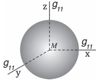
Figure 8. Schematic illustration of how gravity in the x direction has an equal value in the orthogonal y and z directions.
