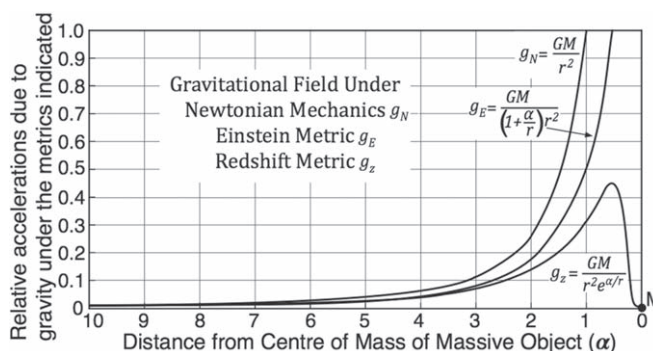
Figure 9. Plots of the relative accelerations due to gravity under Newton's theory, Einstein's metric and this redshift study metric.
