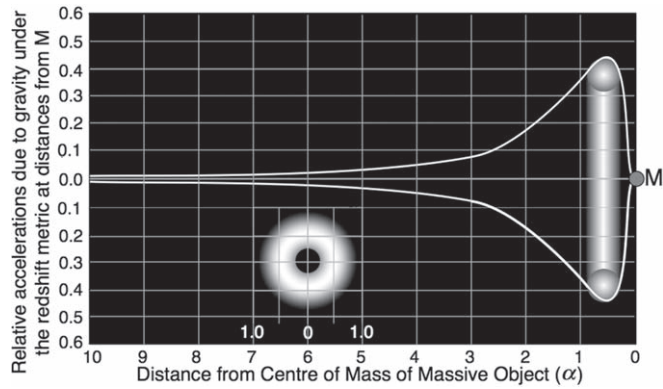
Figure 7. A two dimensional representations of the relative accelerations due to gravity under the redshift metric. The insert shows the expected torus distribution of radiation emitted from an accretion disk that would accumulate around r \approx 0.5\alpha .
