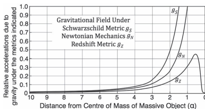
Figure 5. Plots of the relative accelerations due to gravity under the different equations given in table 3.
